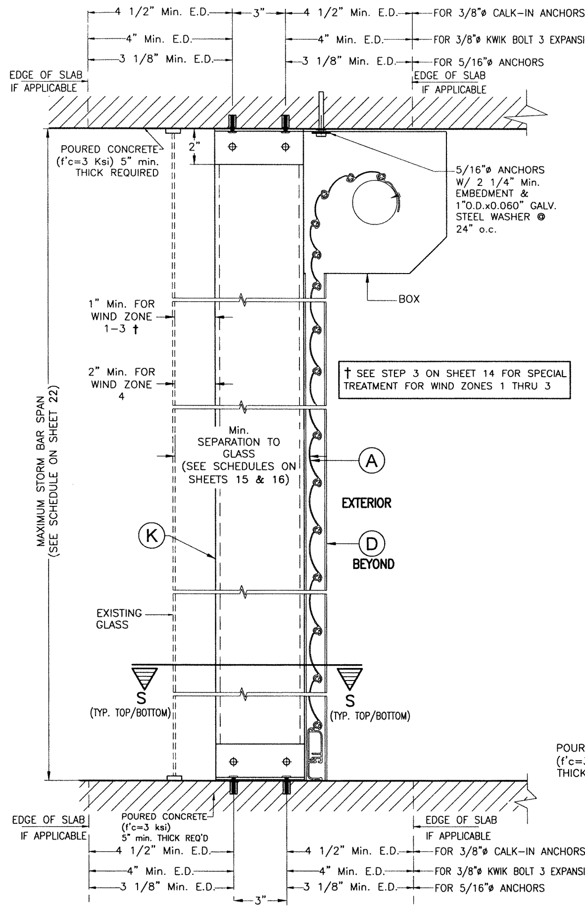
FLOOR TO CEILING / TRAPPED AND WALL MOUNTING: STORM BAR (K) SECTIONS V SCALE: 3/16" = 1"
