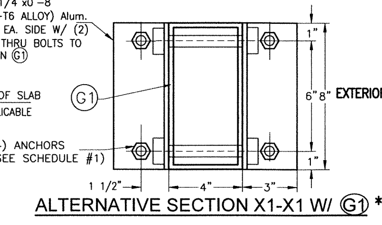
ALTERNATIVE SECTION X1-X1 W/ (G1)* (4"x8" INTERIOR AND END MULLION ONLY W/ ORIENTATION # 1)
