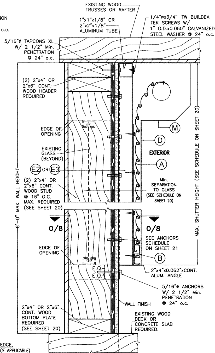
BUILD-OUT MOUNTING
