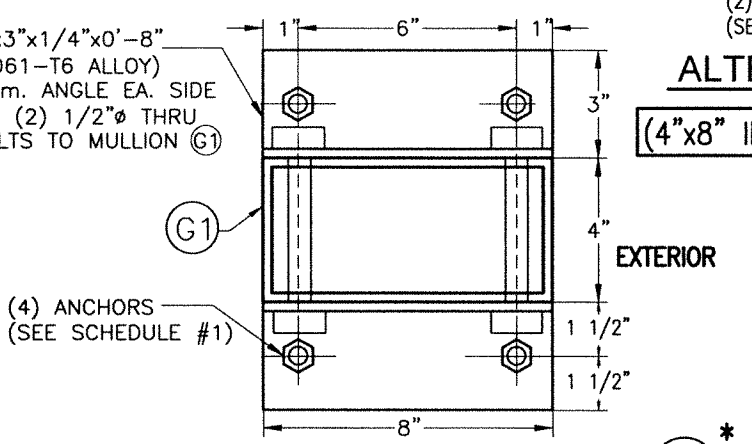
ALTERNATIVE SECTION X1-X1 W/ (G1)* (4"x8" INTERIOR MULLION ONLY W/ ORIENTATION # 2)
