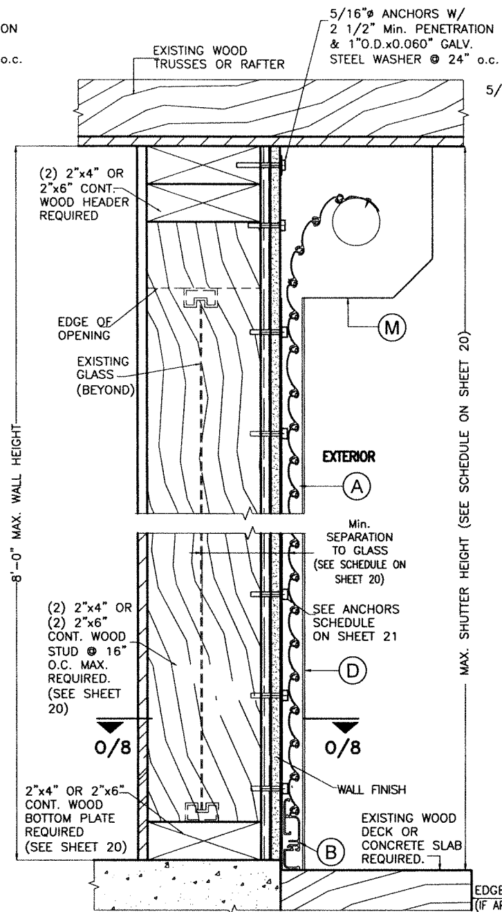
WALL MOUNTING
