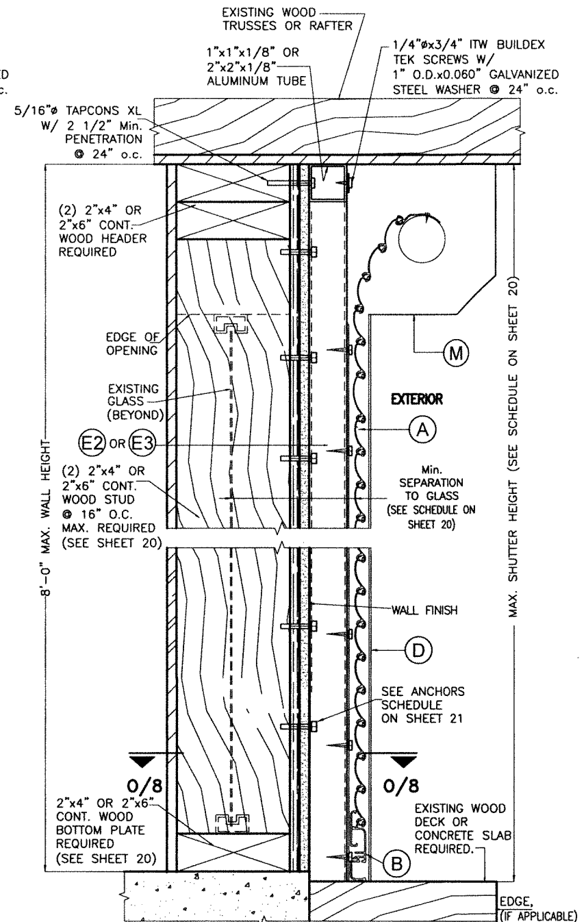
BUILD-OUT MOUNTING
