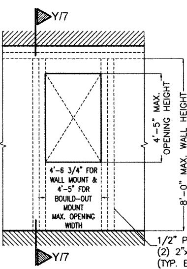
DETAIL 1 (ELEVATION)
