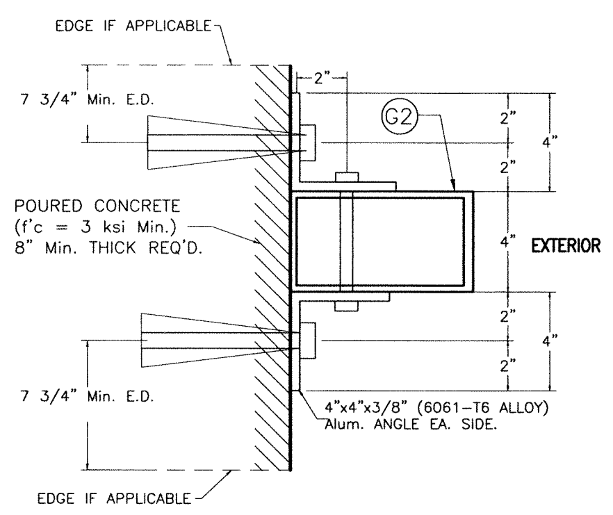
SECTION X4-X4 W/ G2 * (END & INTERIOR MULLION) (W/ ORIENTATION # 2) (4"x7")
