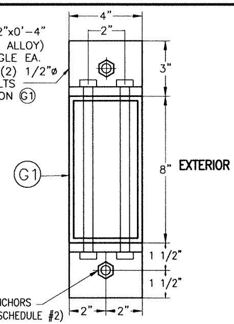
ALTERNATIVE SECTION X1-X1 W/ (G1)* (4"x8" INTERIOR AND END MULLION W/ ORIENTATION # 1)
