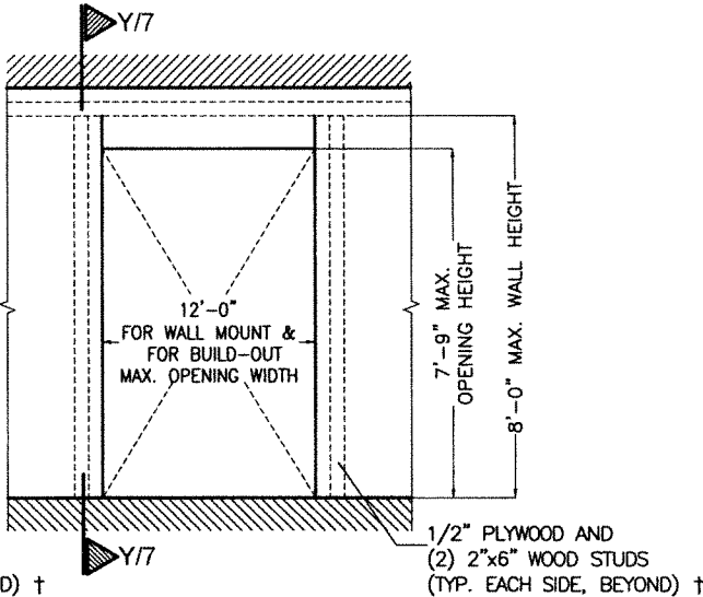
DETAIL 2 (ELEVATION)
