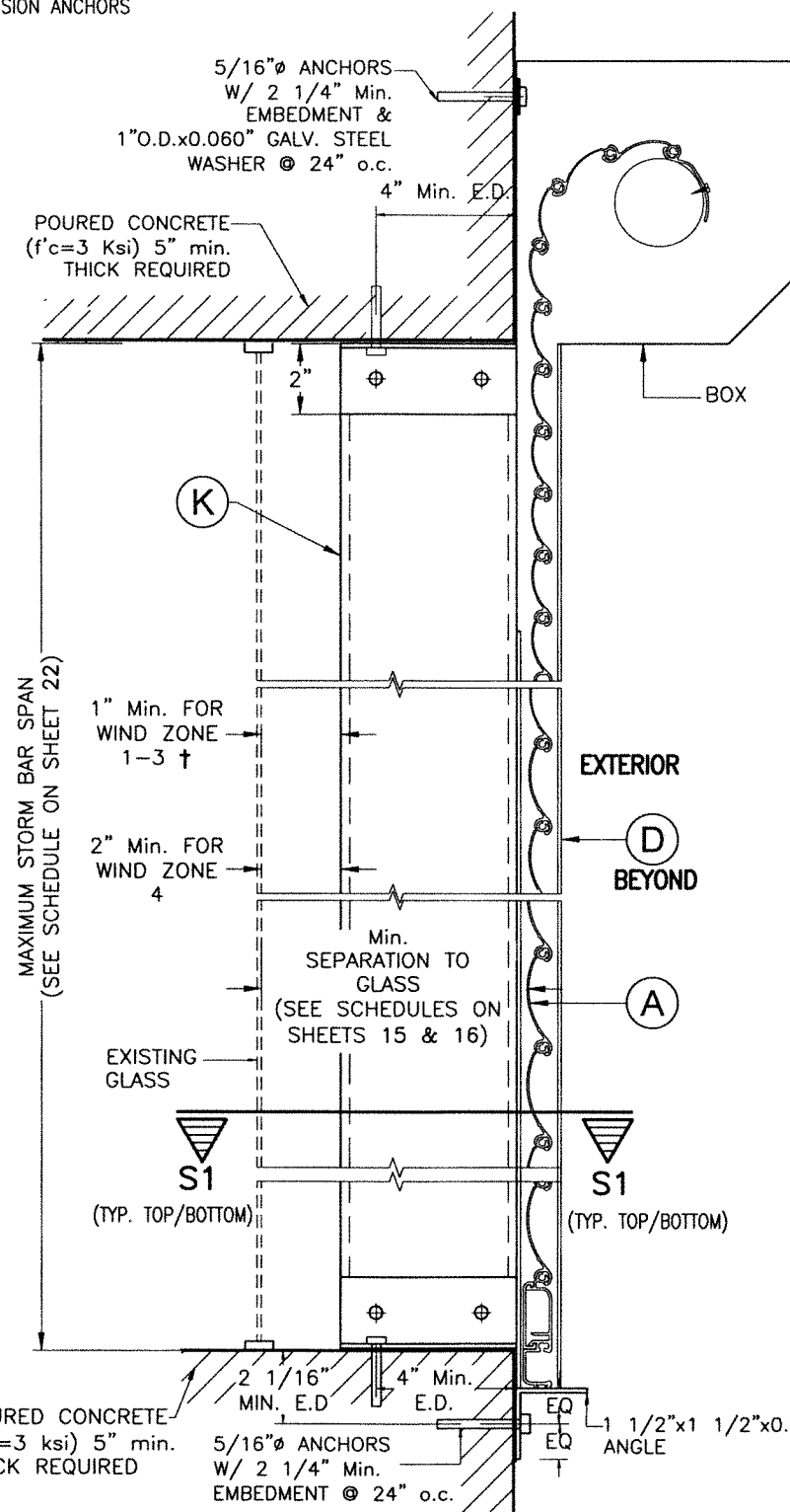
WALL MOUNTING
